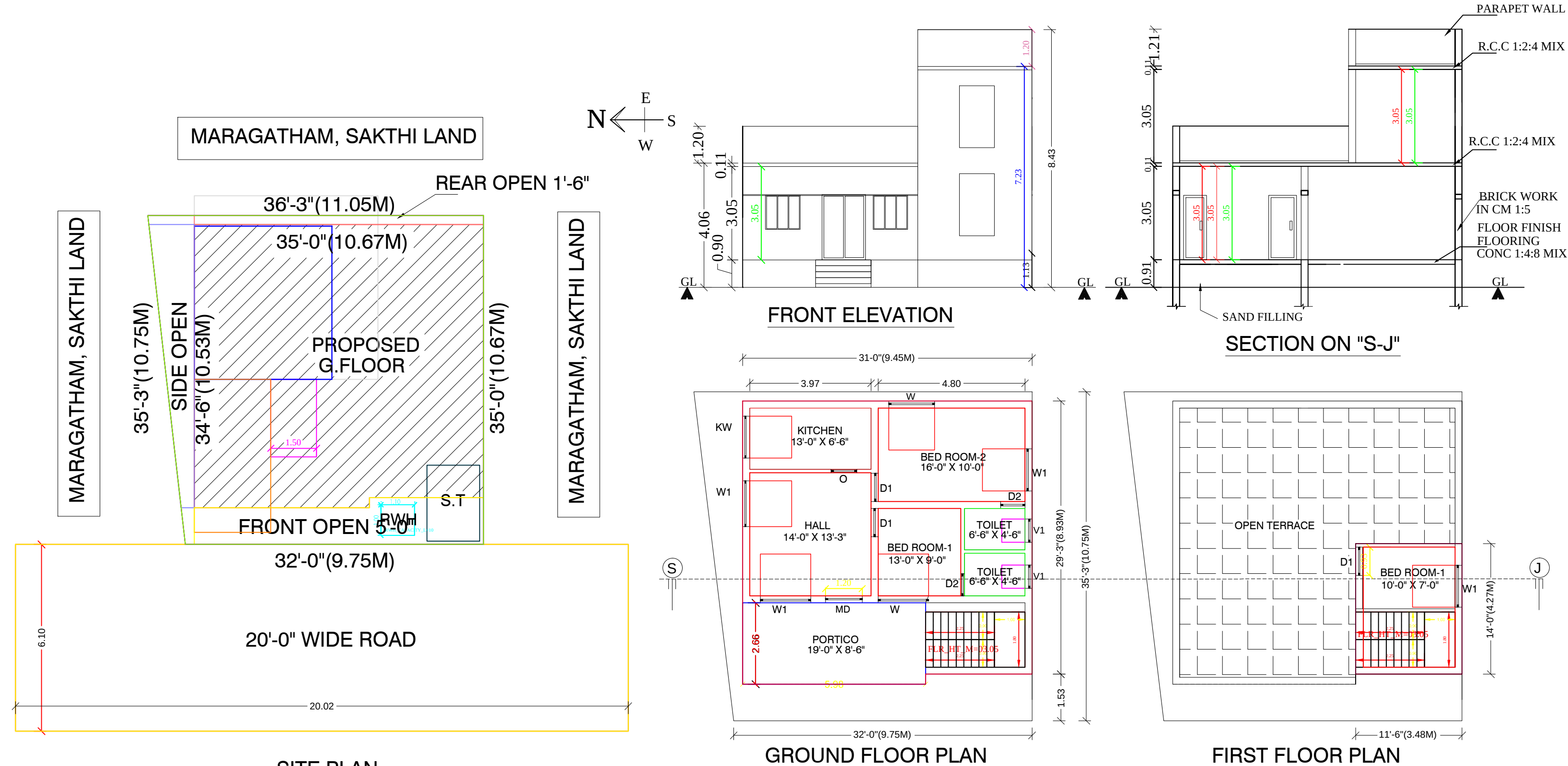
SITE PLAN SCALE: 1CM : 1M
