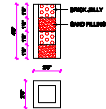
PERCOLATION PIT
