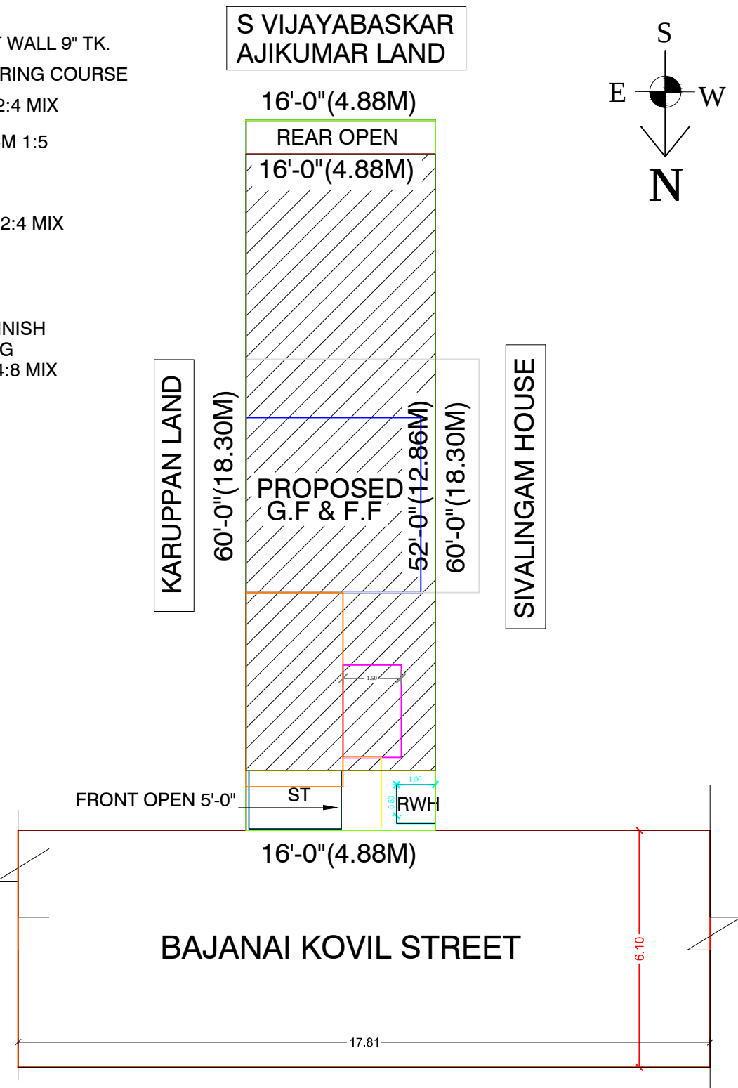
SITE PLAN
