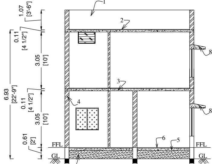
SECTION ON "JS"
