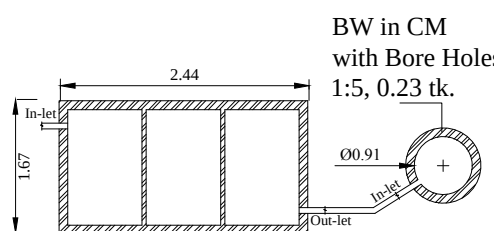
(1.98x1.21x2.10M) PLAN - SEPTIC TANK & SOAK PIT
