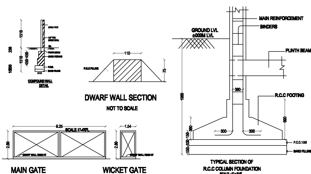
MAIN GATE, WICKET GATE, and TYPICAL SECTION OF R.C.C COLUMN FOUNDATION
