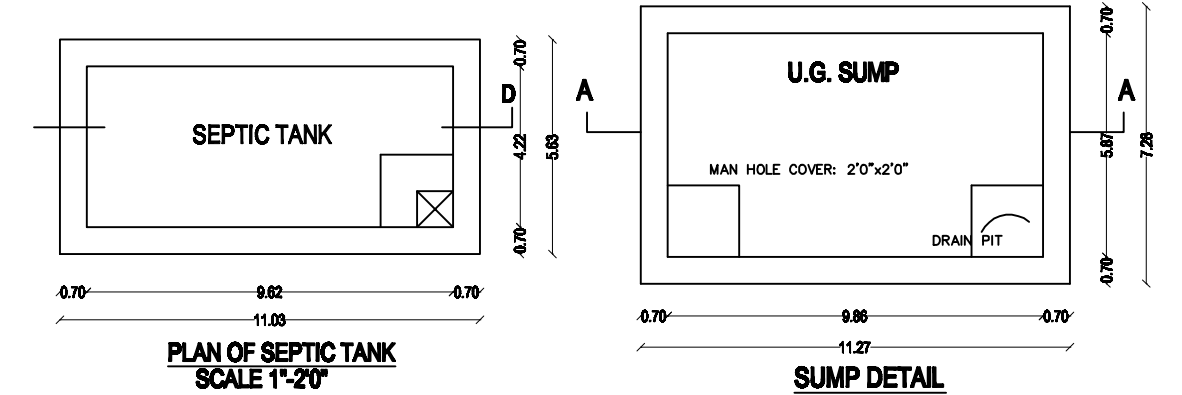
SEPTIC TANK and U.G. SUMP
