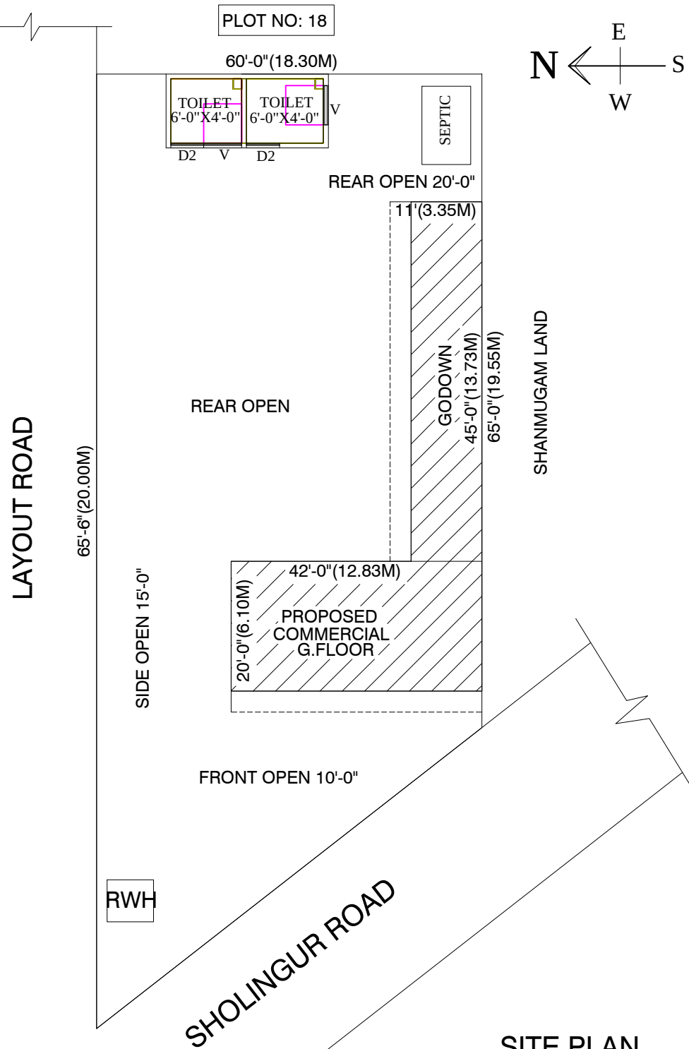
SITE PLAN
