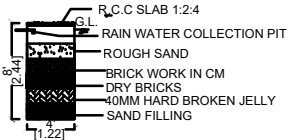
RAIN WATER HARVEST UNIT
