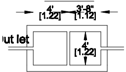
Plan SEPTIC TANK DETAIL
