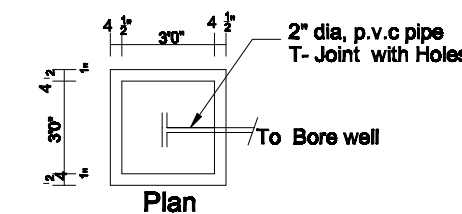
RAINWATER HARVESTING TANK SCALE 1:50
