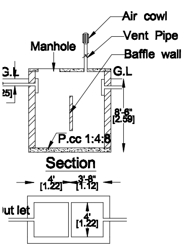
Plan SEPTIC TANK DETAIL
