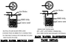
RAIN WATER HARVESTING TANK DETAIL
