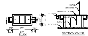
SECTION ON JS1 PLAN
