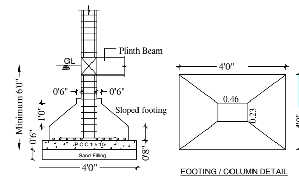
COLUMN DETAILS
