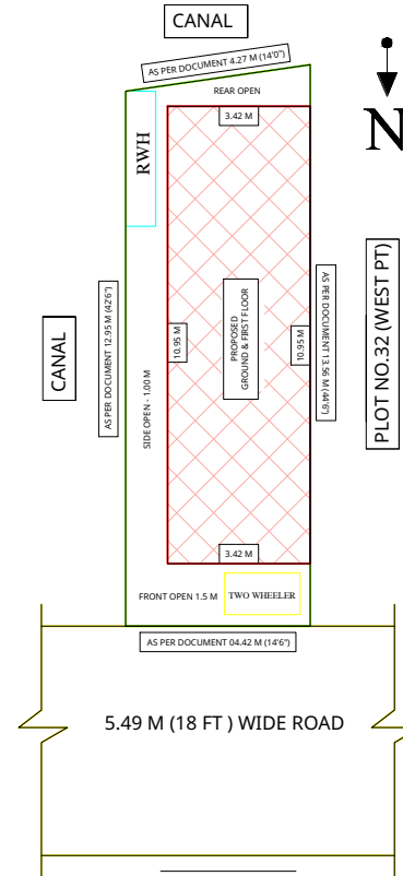
SITE PLAN
