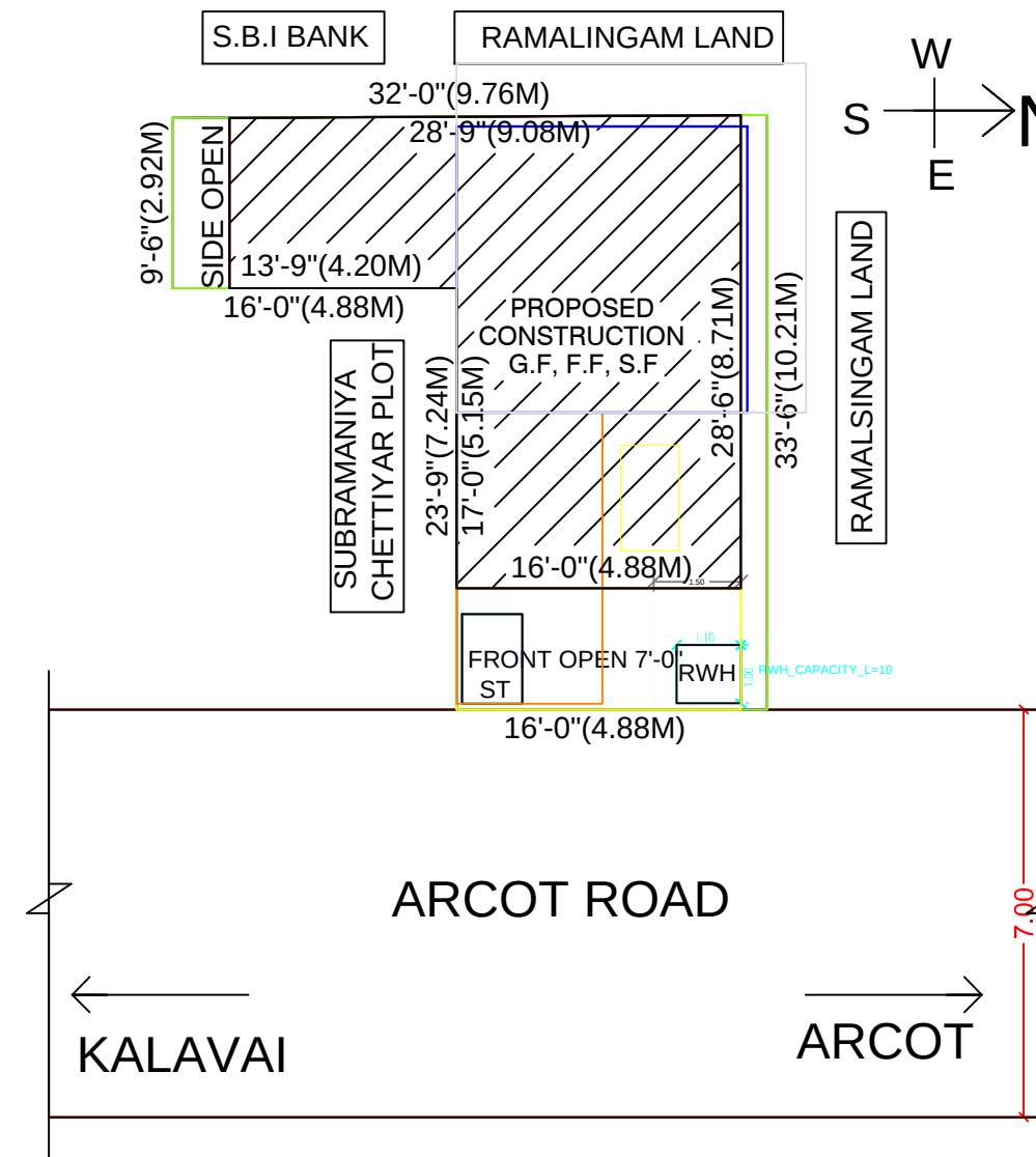
SITE PLAN (SCALE: 1CM : 1M)
