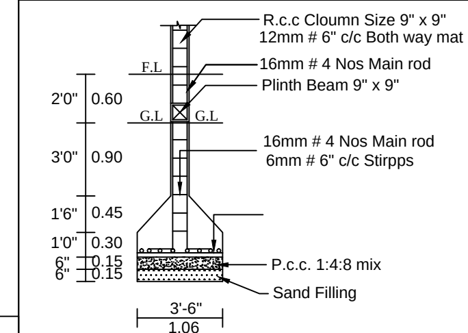
COLUMN DETAIL NOT TO SCALE
