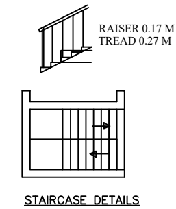
STAIRCASE DETAILS
