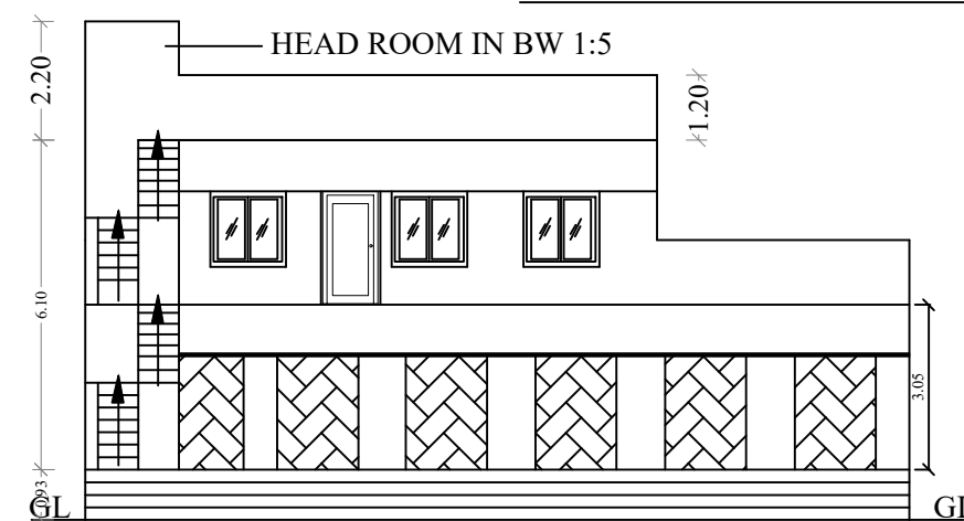
FRONT ELEVATION
