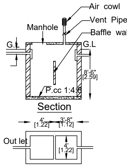
Plan SEPTIC TANK DETAIL
