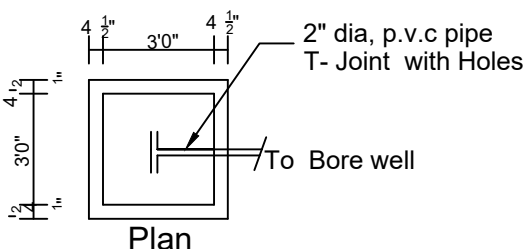
RAINWATER HARVESTING TANK SCALE 1:50
