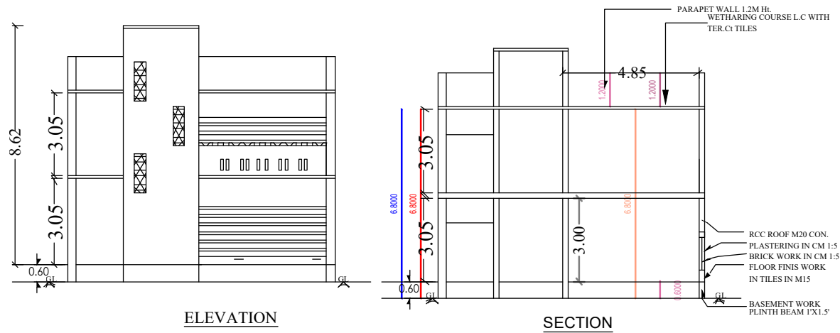
SECTION
