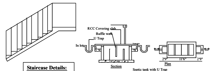
Staircase Details: Rise : 0.15m Tread: 0.25m Width : 1.0m Height : 1.25 m
