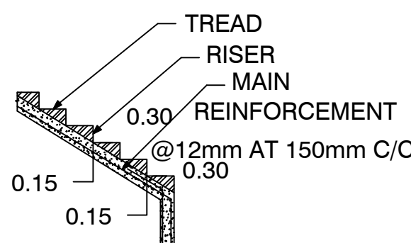
STAIRCASE DETAILS NOT TO SCALE
