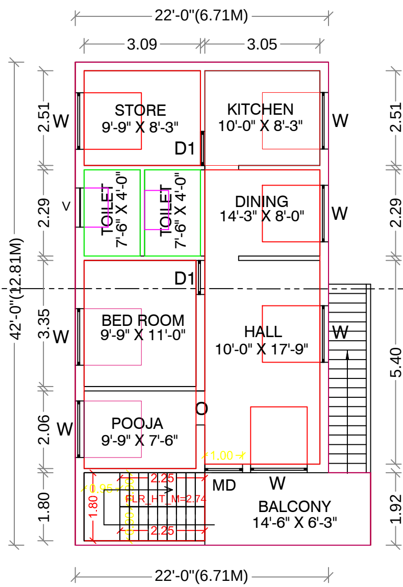
PROPSOED ADDITIONAL FIRST FLOOR PLAN
