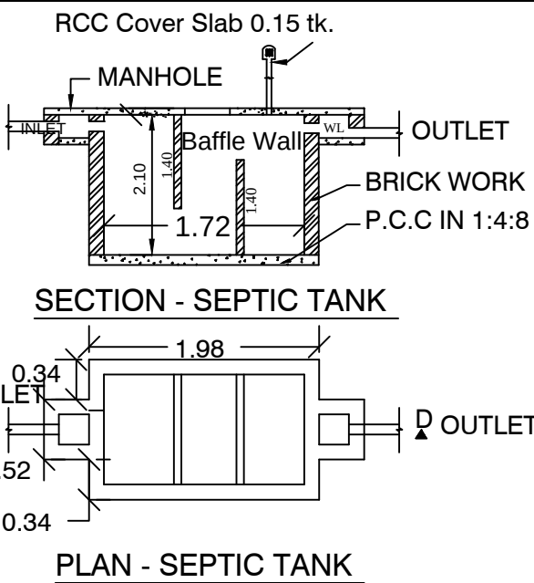
PLAN - SEPTIC TANK
