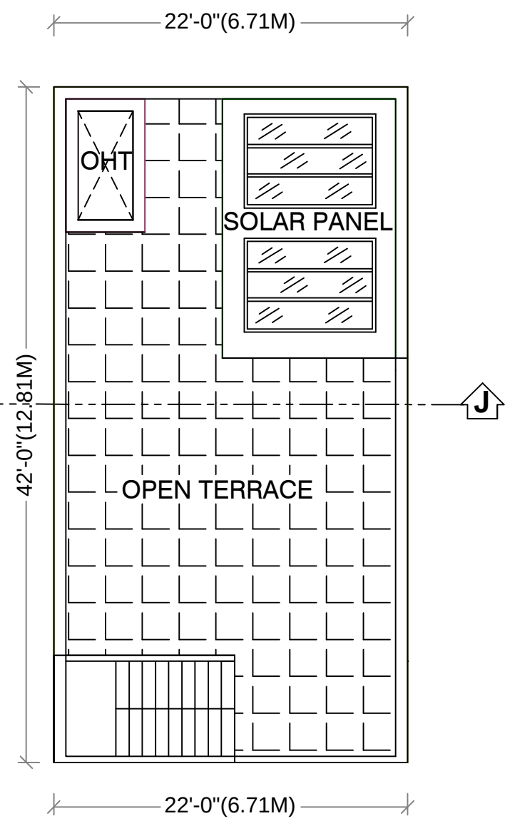
HEAD ROOM & TERRACE FLOOR PLAN
