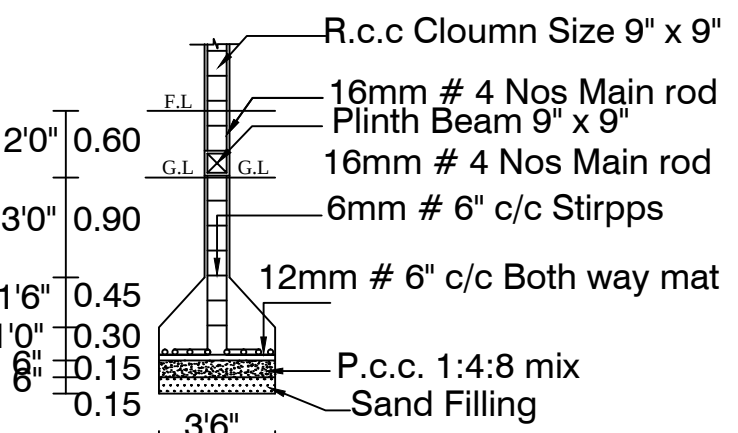
COLUMN DETIAL
