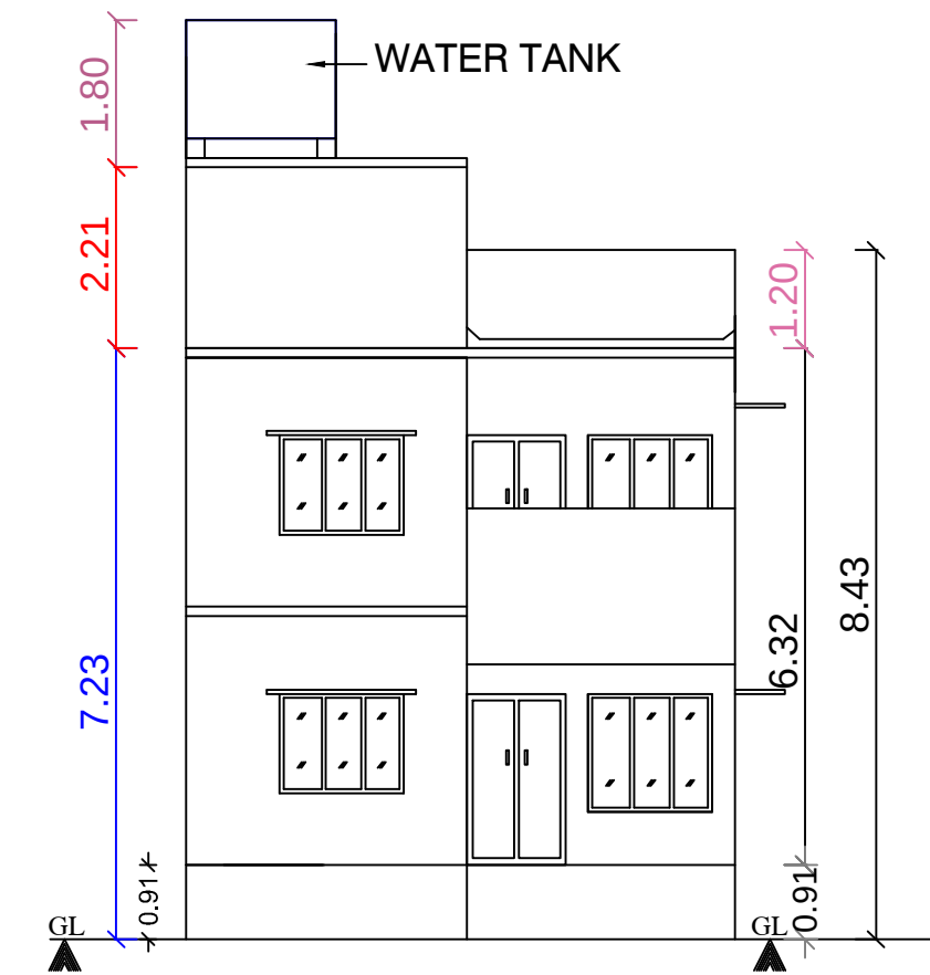
FRONT ELEVATION
