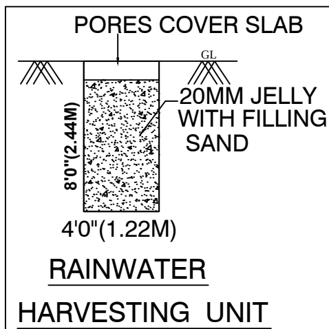
PORES COVER SLAB 20MM JELLY WITH FILLING SAND RAINWATER HARVESTING UNIT
