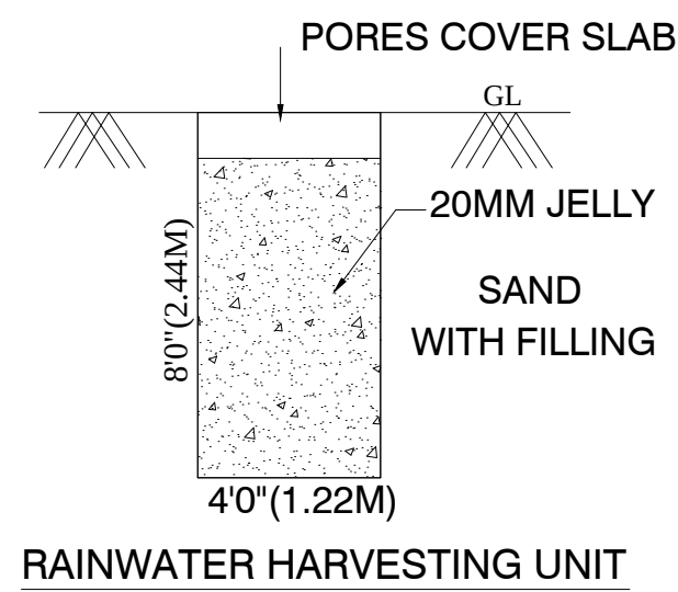
RAINWATER HARVESTING UNIT
