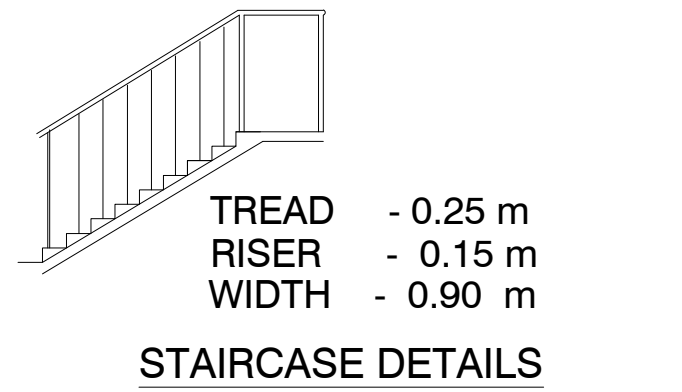
STAIRCASE DETAILS
