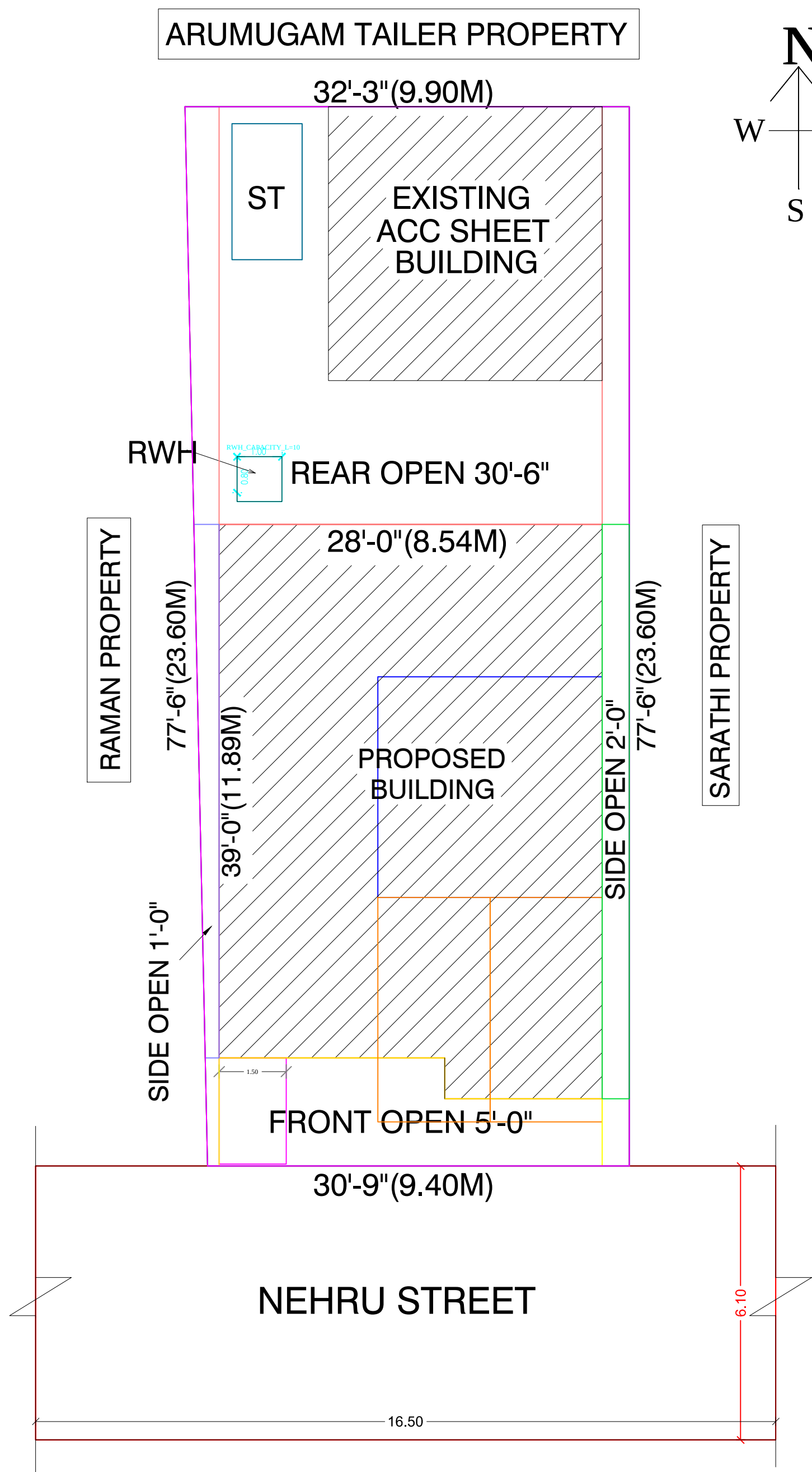
SITE PLAN (SCALE: 1CM : 1M)
