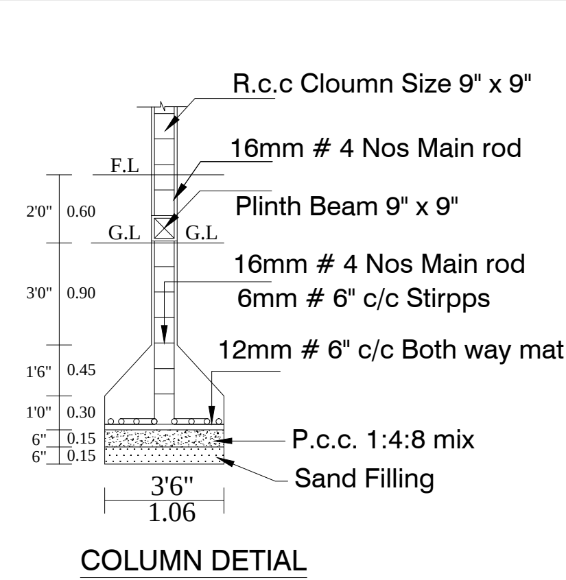
COLUMN DETIAL
