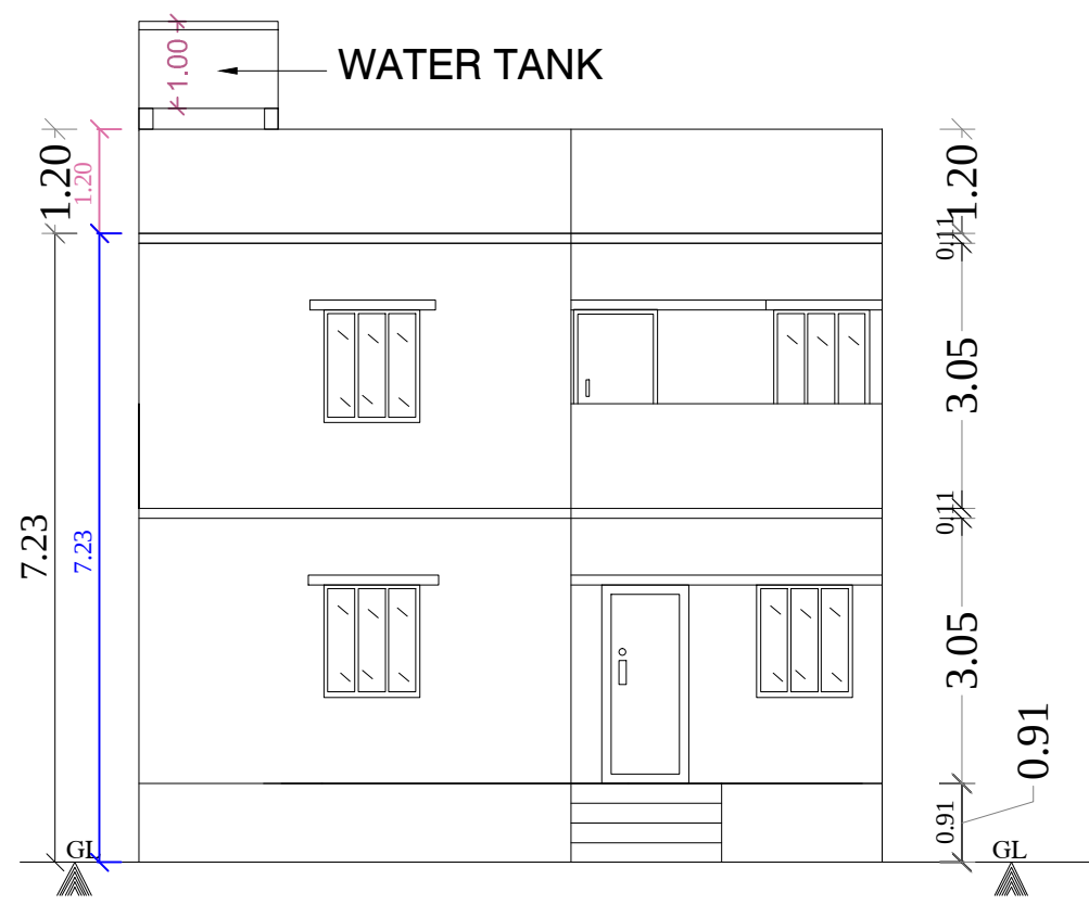
FRONT ELEVATION
