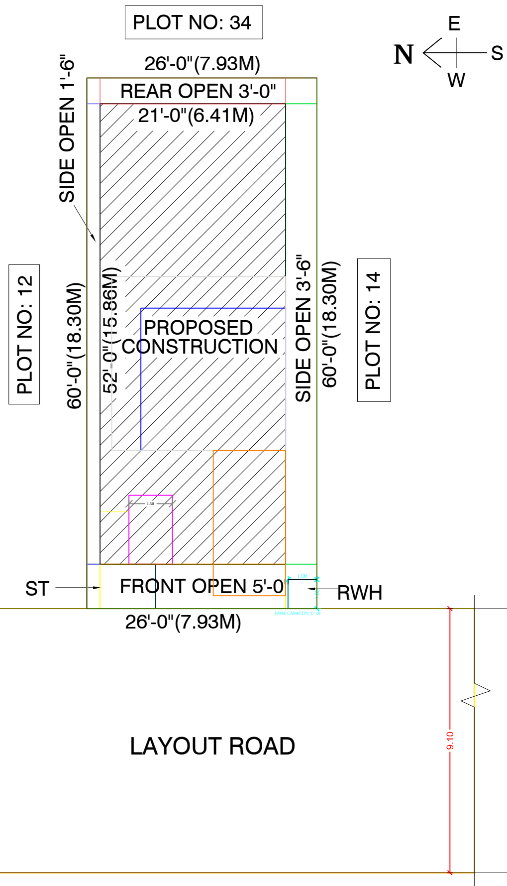
SITE PLAN SCALE : 1CM =1M
