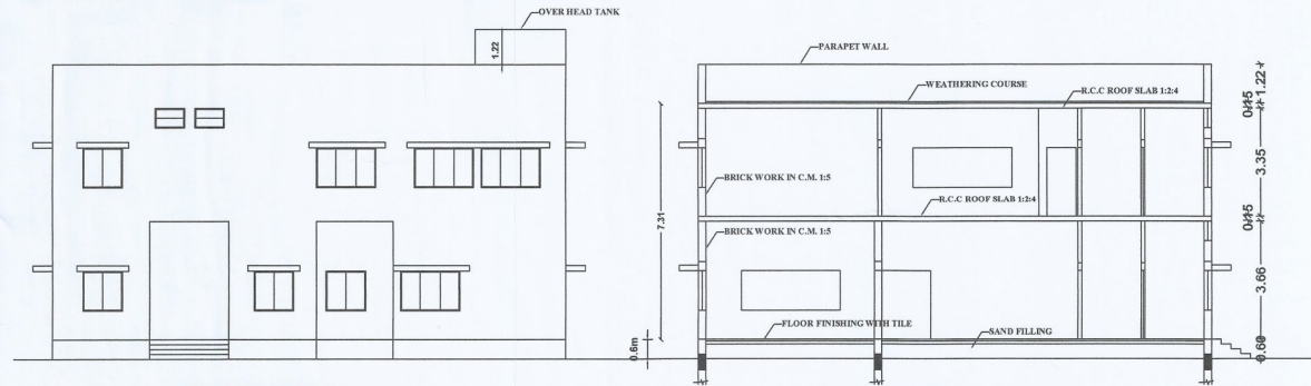
SECTION ON X-X
