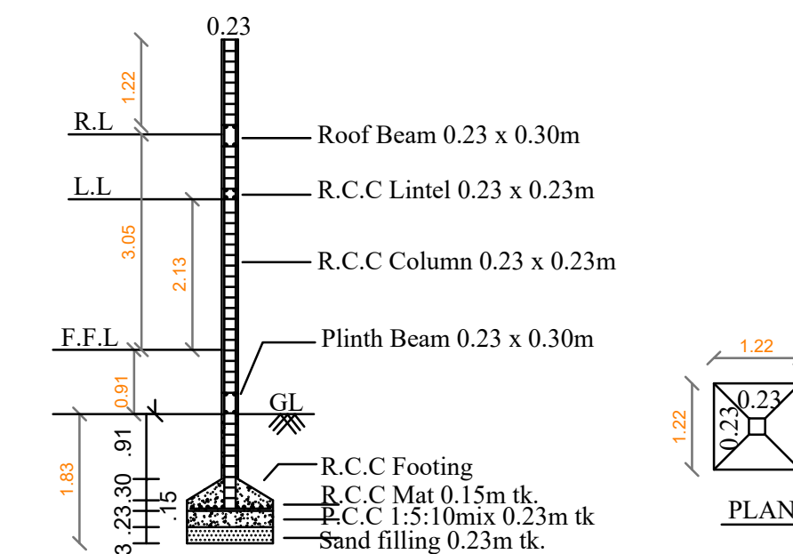
SECTION R.C.C FOUNDATION AND COLUMN DETAILS
