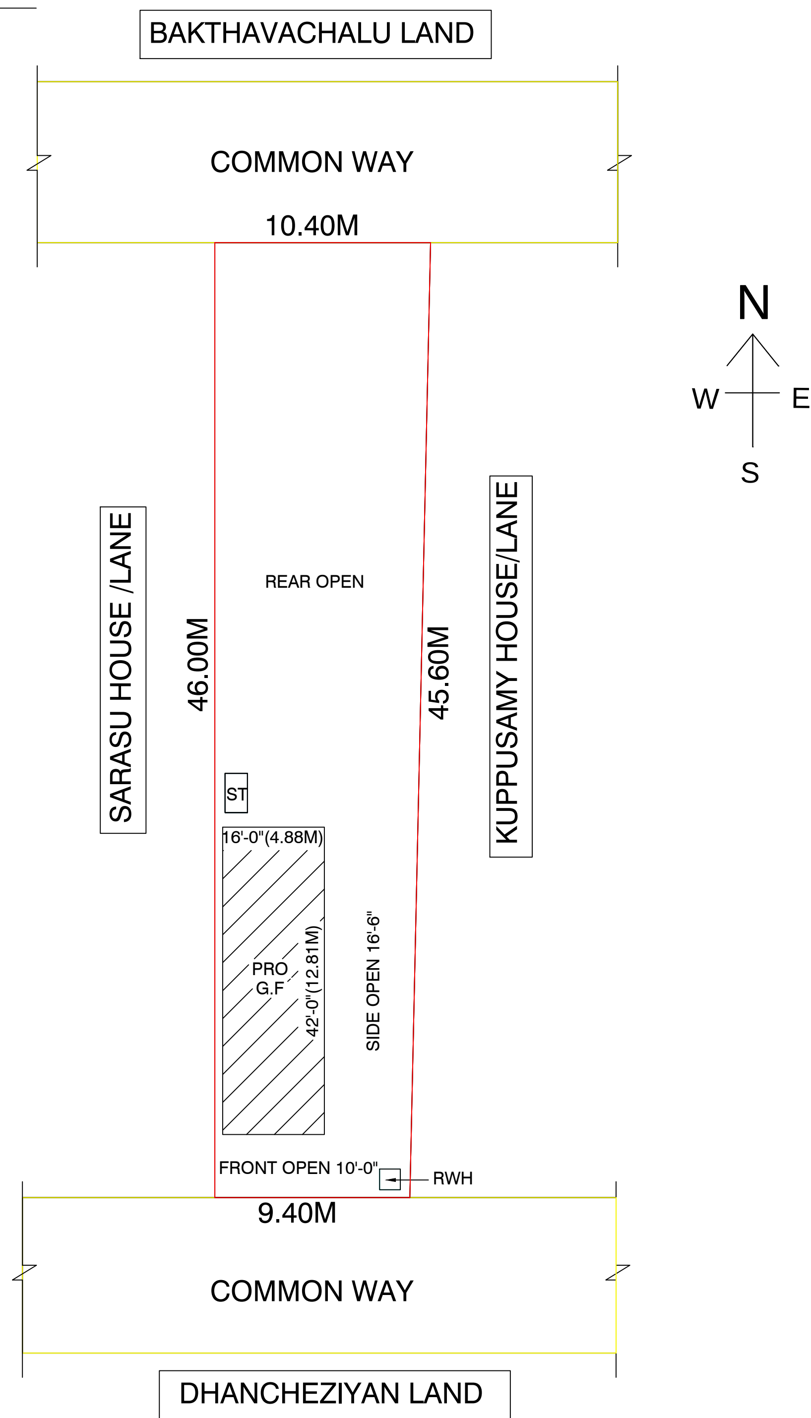
SITE PLAN (SCALE: 1CM : 2M)
