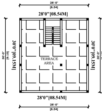
TERRACE FLOOR
