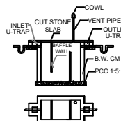
SEPTIC TANK DETAILS SIZE: 6'0" x 3'0" x 6'0"
