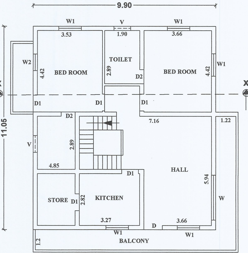
SECOND FLOOR PLAN ( PROPOSED ADDITIONAL CONSTRUCTION )
