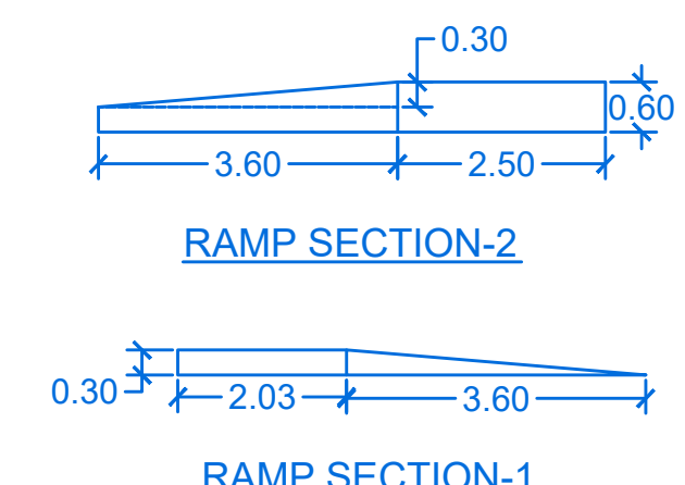
RAMP SECTION-
