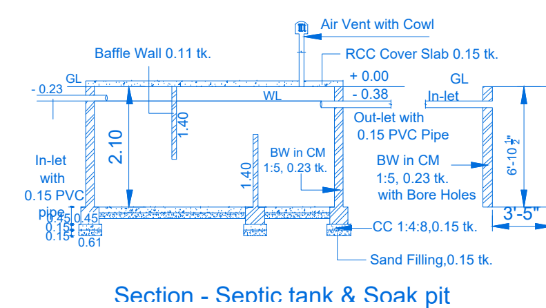
Section - Sentic tank &amp; S
