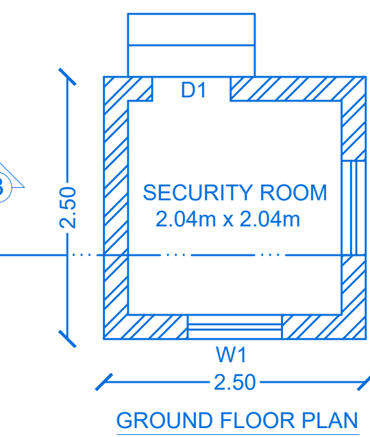
FUND FLOOR PLAN
