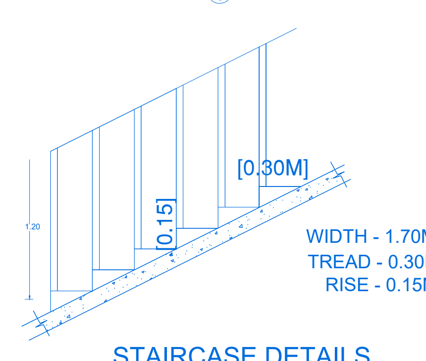
STAIRCASE DETAILS
