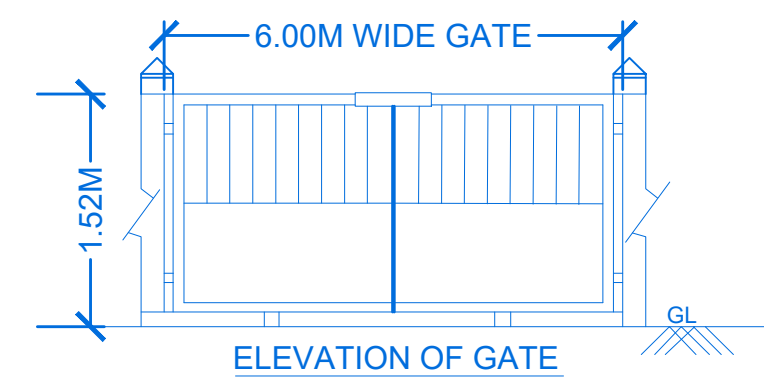
ELEVATION OF GATE
