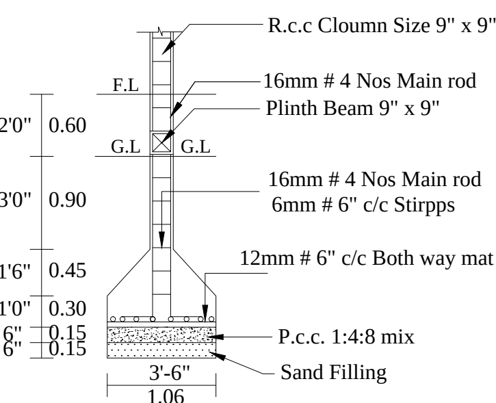
COLUMN DETIAL
