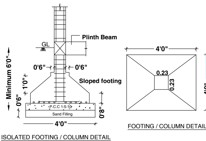
COLUMN DETAILS
