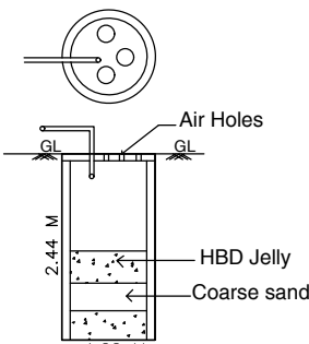
RAIN WATER HARVESTING TANK DETAIL
