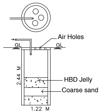
WASTE WATER RECYLING TANK DETAIL
