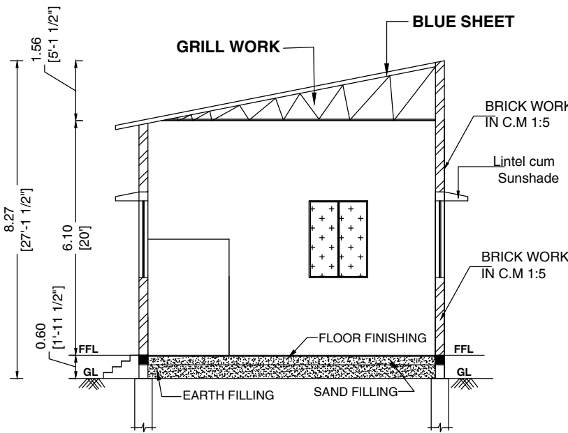
SECTION ON "JS"
