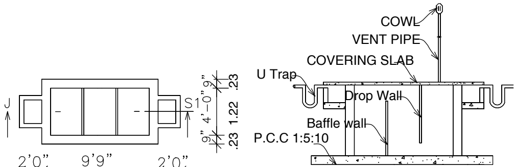
SECTION ON JS1
