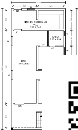
PRO. GROUND
