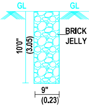
PERCOLATION PIT
