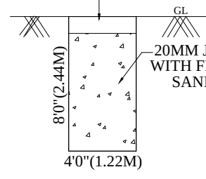
RAIN WATER HARVESTING UNIT
