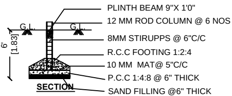
SECTION FOUNDATION DETAILS
