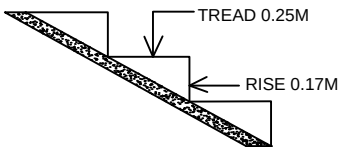
STAIR DETAILS
