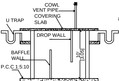
SECTION FOUNDATION DETAILS
