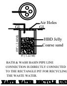
BATH & WASH BASIN PIPE LINE CONNECTION IS DIRECTLY CONNECTED TO THE RECTANGLE PIT FOR RECYCLING THE WASTE WATER.
