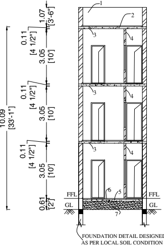
SECTION ON "J-S"
