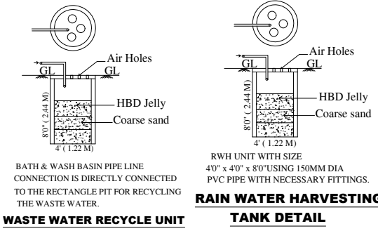
WASTE WATER RECYCLE UNIT
