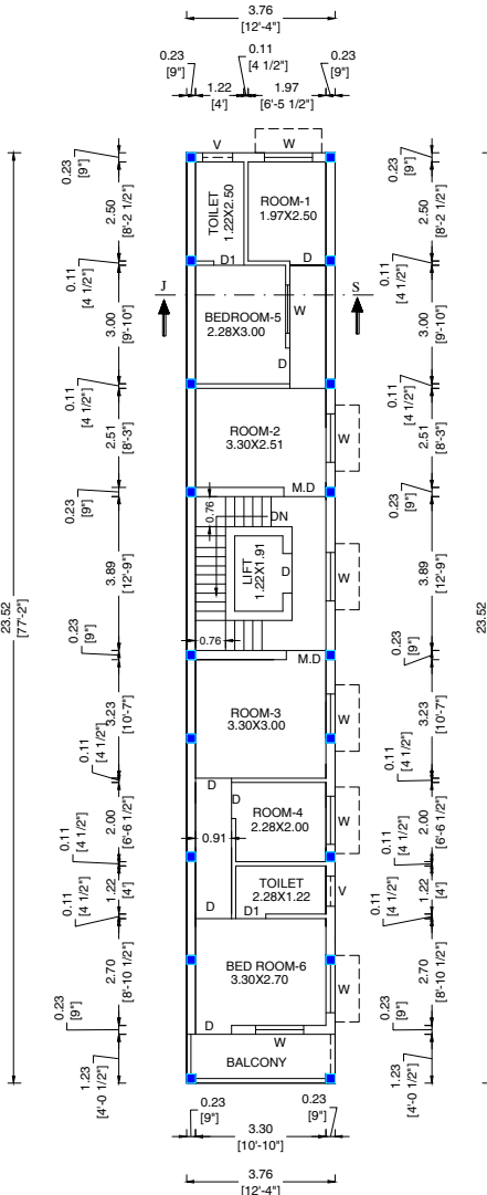
PRO., SECOND FLOOR PLAN
