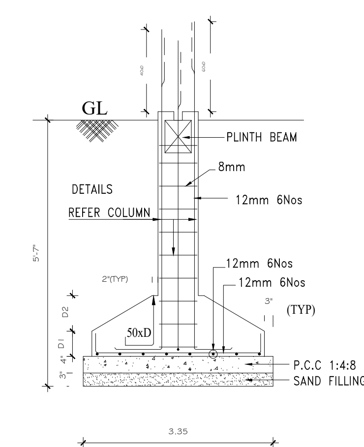
FOUNDATION DETAILS (NOT TO SCALE)
