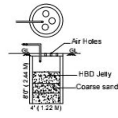
RAIN WATER HARVESTING TANK DETAIL
