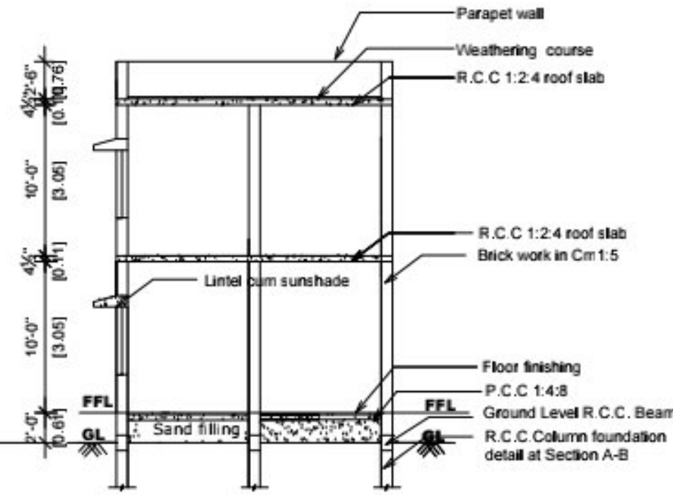
SECTION ON 'RK'
