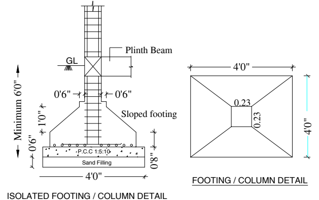
COLUMN DETAILS
