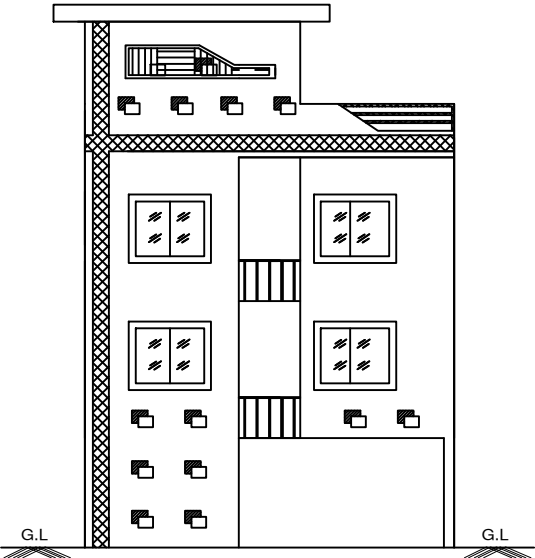
FRONT ELEVATION
