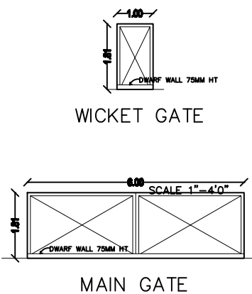
GATE DETAILS
