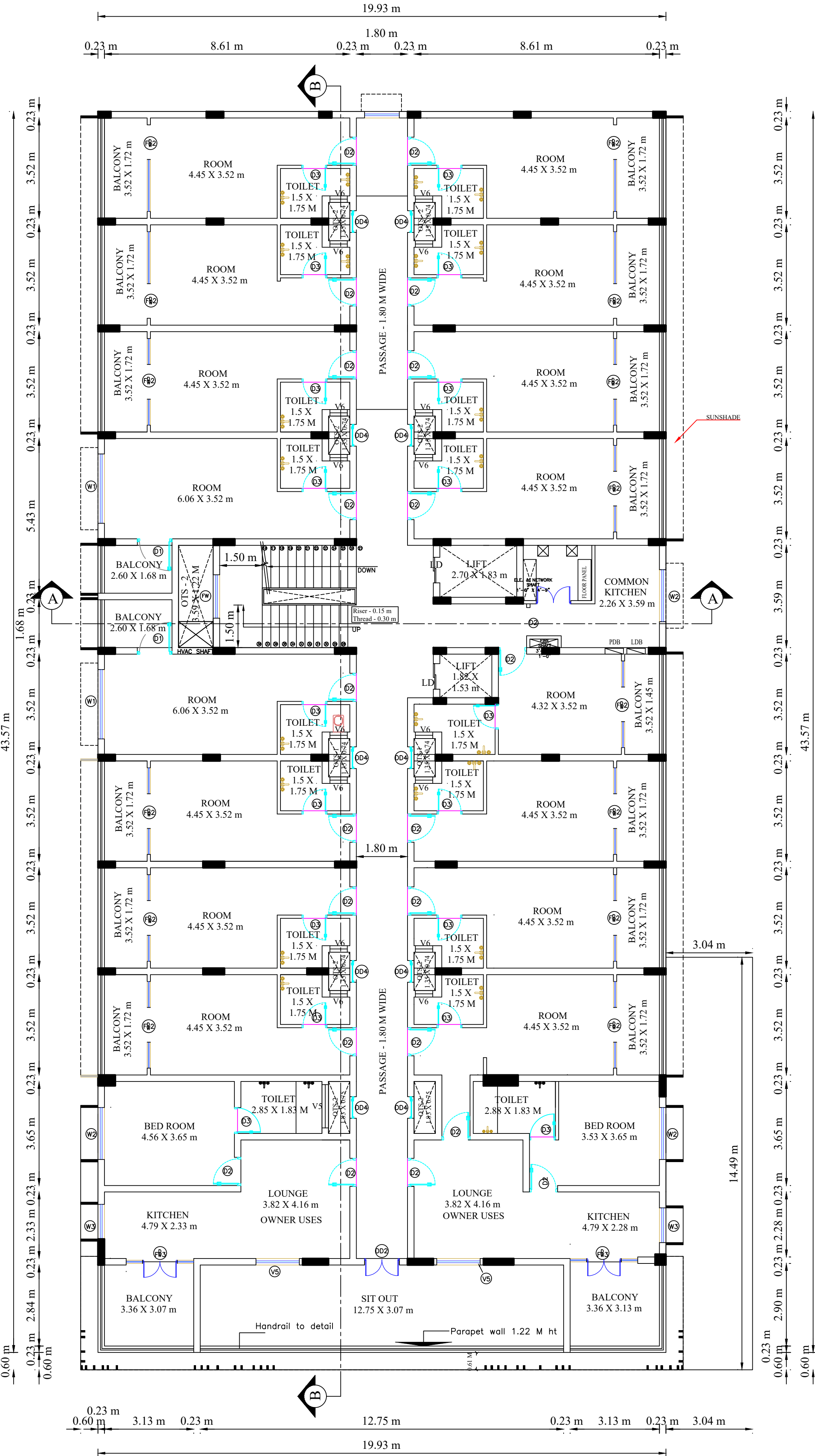
TYPICAL FLOOR PLAN (1st,2nd,3rd and 4th)
