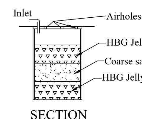
RAIN WATER HARVESTING UNIT (NOT TO SCALE)
