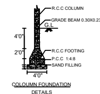
COLOUMN FOUNDATION DETAILS
