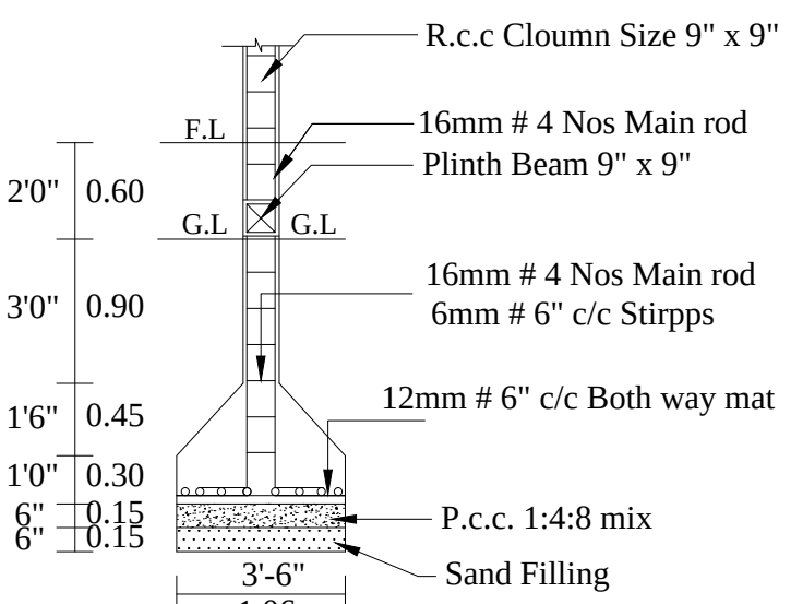
COLUMN DETIAL
