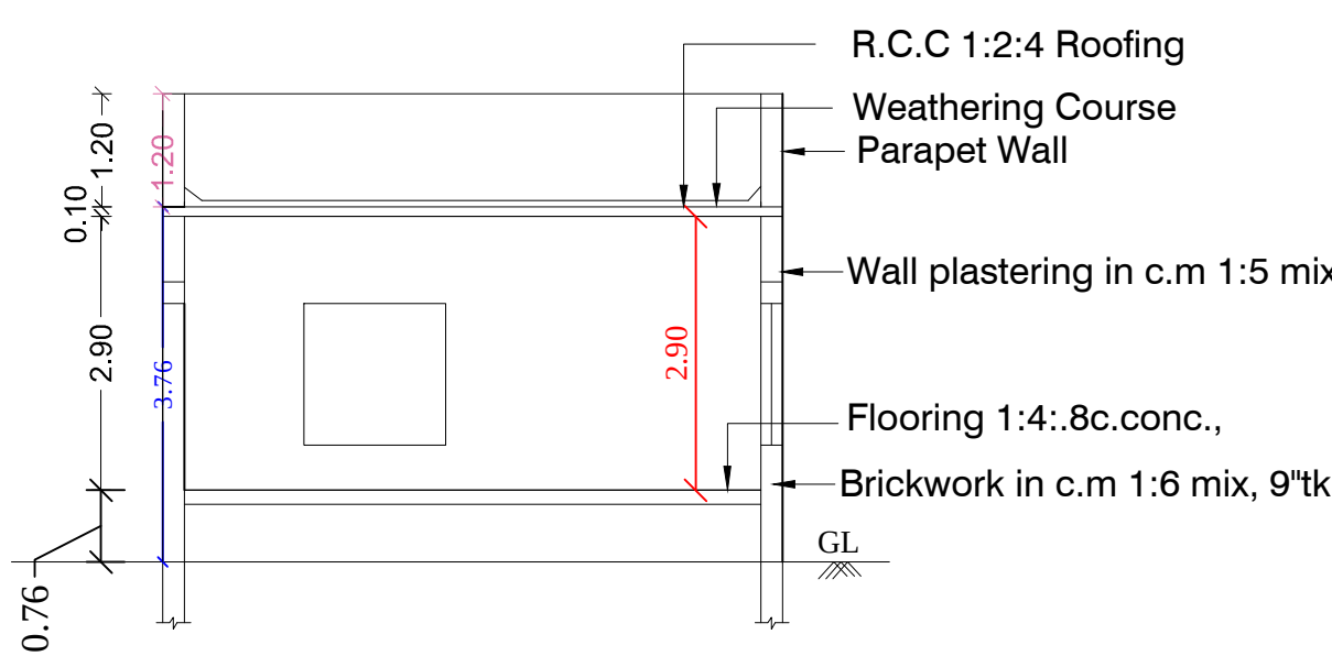
SECTION ON JJ
