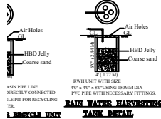
RAINWATER HARVESTING UNIT
