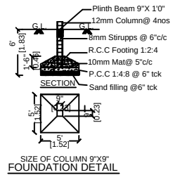
SIZE OF COLUMN 9"X9" FOUNDATION DETAIL
