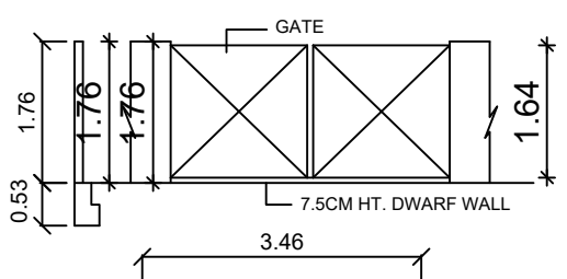
COMPOUND WALL WITH DWARF WALL DETAILS
