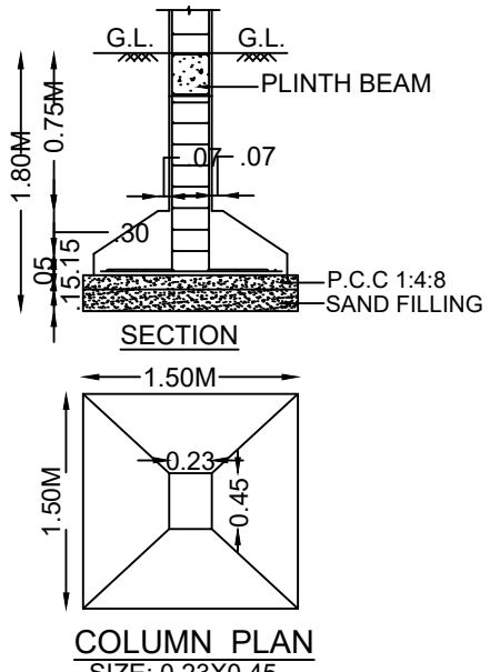
TYPICAL FOUNDATION DETAIL
