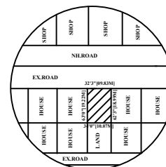
TOPO PLAN.
