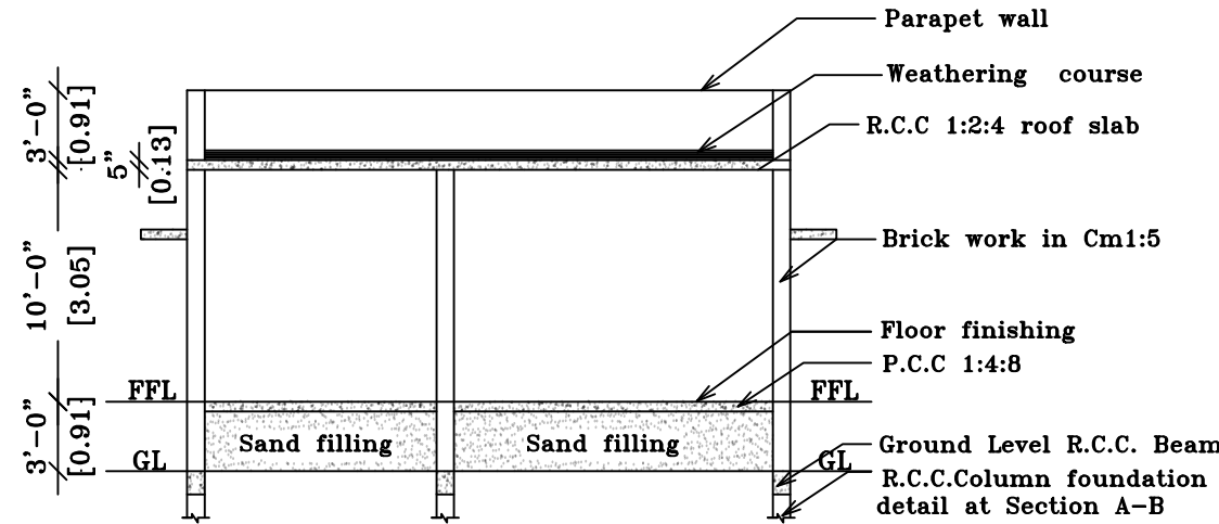
SECTION ON 'SA'
