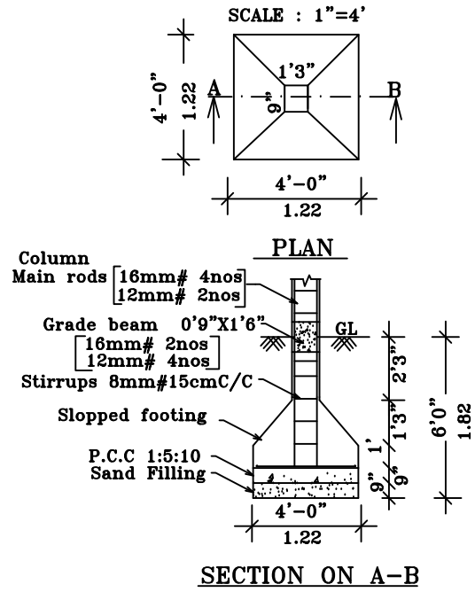
COLUMN DETAILS
