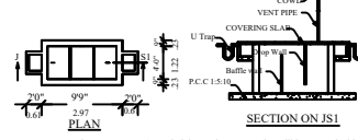
SEPTIC TANK DETAILS Using 'U' type trap 2 Nos in inlet, outlet & Vent pipe will be covered with Mosquito proof covering net in inner side and top of vent pipe.
