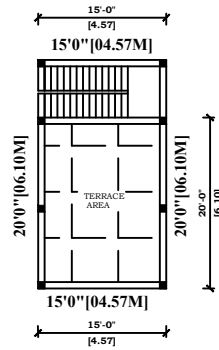
TERRACE FLOOR
