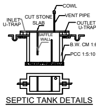
SEPTIC TANK DETAILS SIZE - 6'0" X 3'0" X 6'0"
