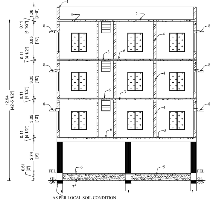
SECTION ON "JS"
