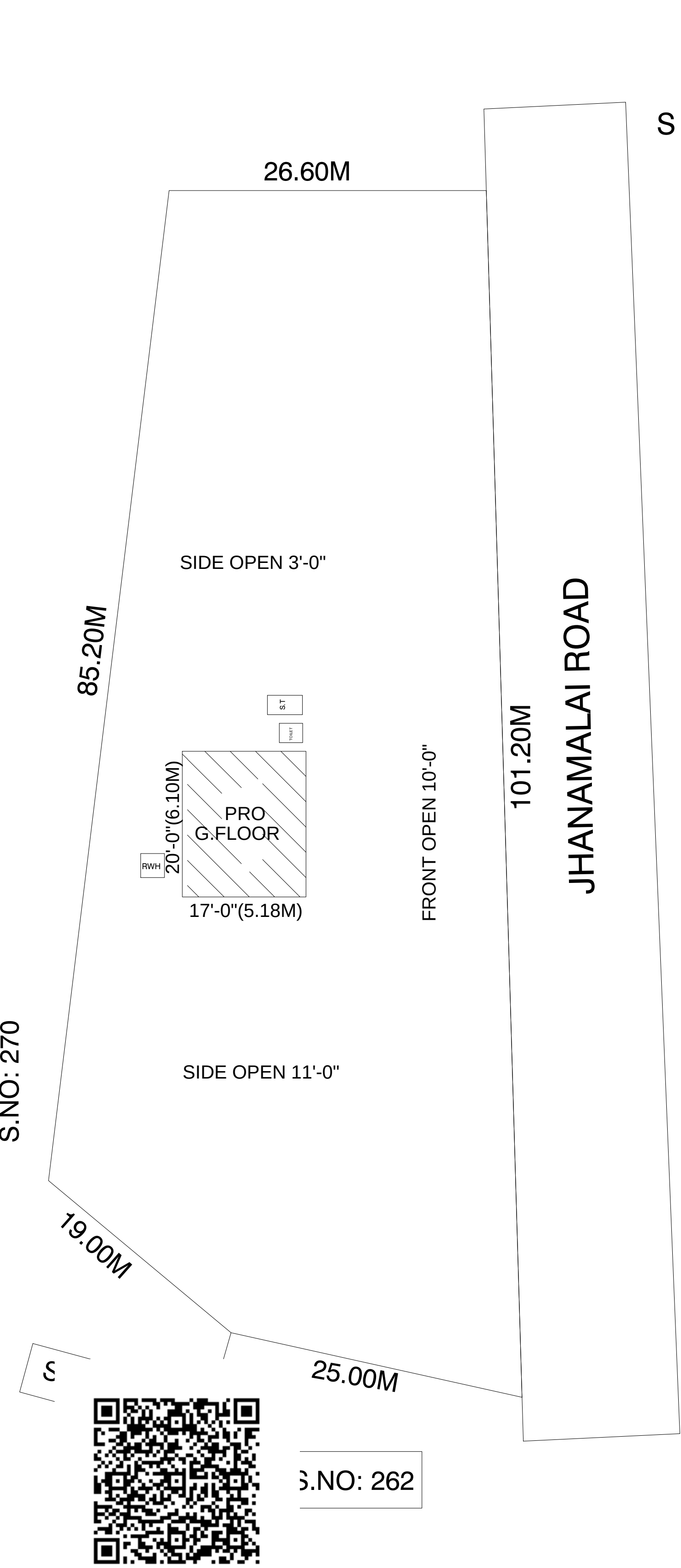
SITE PLAN (SCALE: 1CM : 2M)
